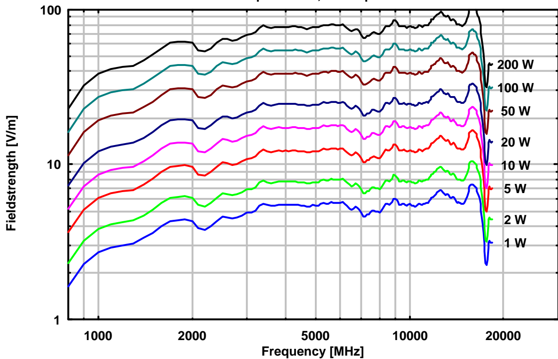
BBHA 9120 D Input Power, Dist. Aperture-EuT: 4 m
