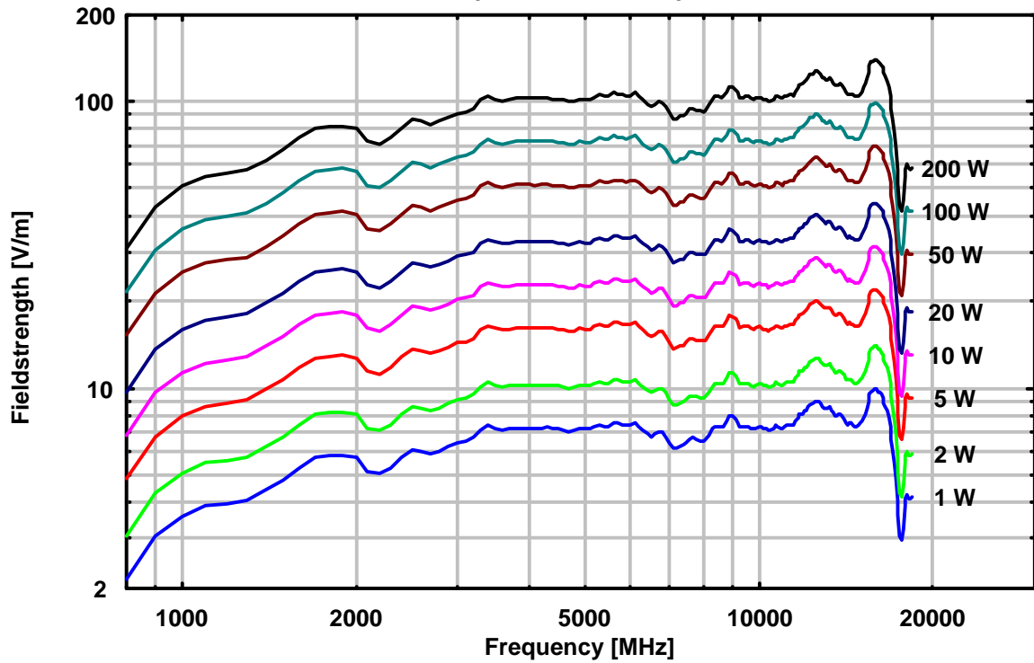
BBHA 9120 D Input Power, Dist. Aperture-EuT: 3 m
