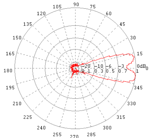
H-Ebene / H-Plane 14 GHz
