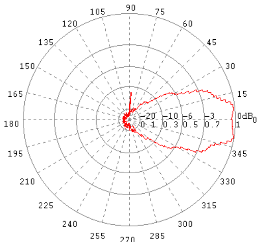
E-Ebene / E-Plane 14 GHz
