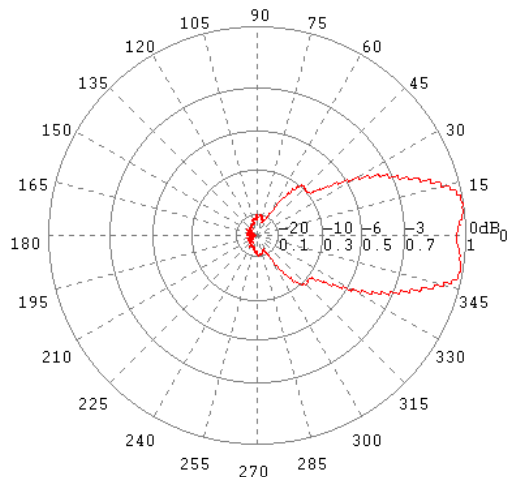
E-Ebene / E-Plane 9 GHz
