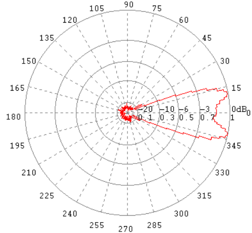
H-Ebene / H-Plane 13 GHz
