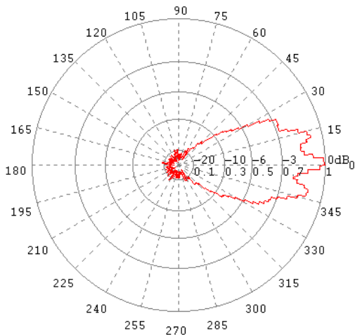
E-Ebene / E-Plane 17 GHz
