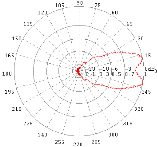
E-Ebene / E-Plane 13 GHz
